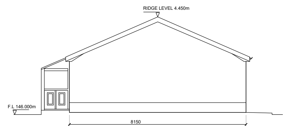
SIDE ELEVATION - EAST FACING SCALE; 1:100
